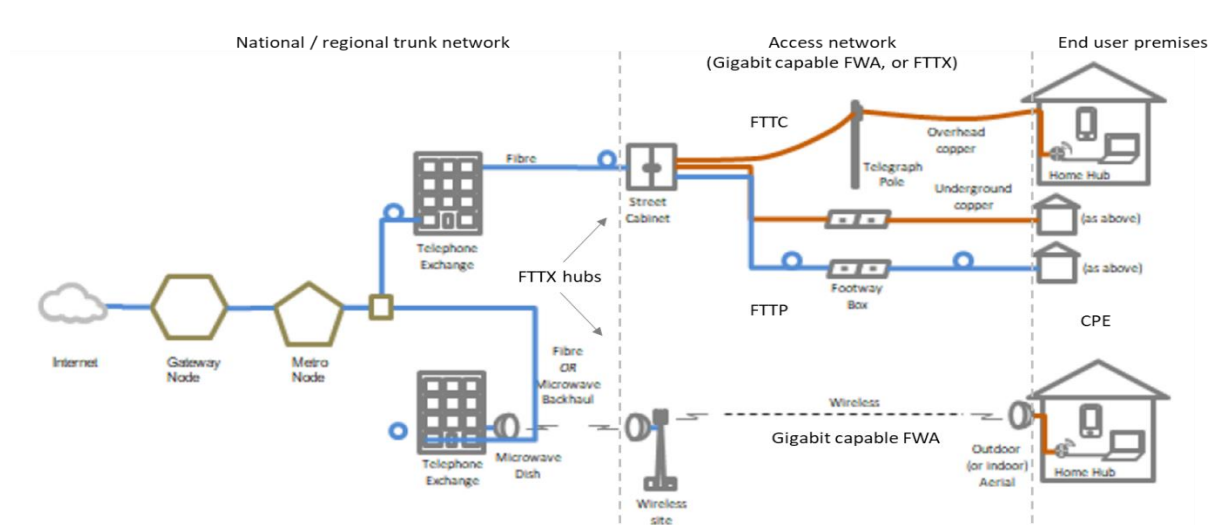
Figure 1.1: Typical access network configurations 1
